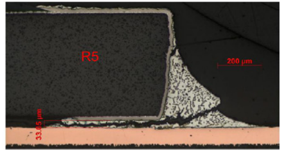
Figure 8: Typical failure diagram from Lui et. al. and a cross-section of the failed R5 solder joint.
