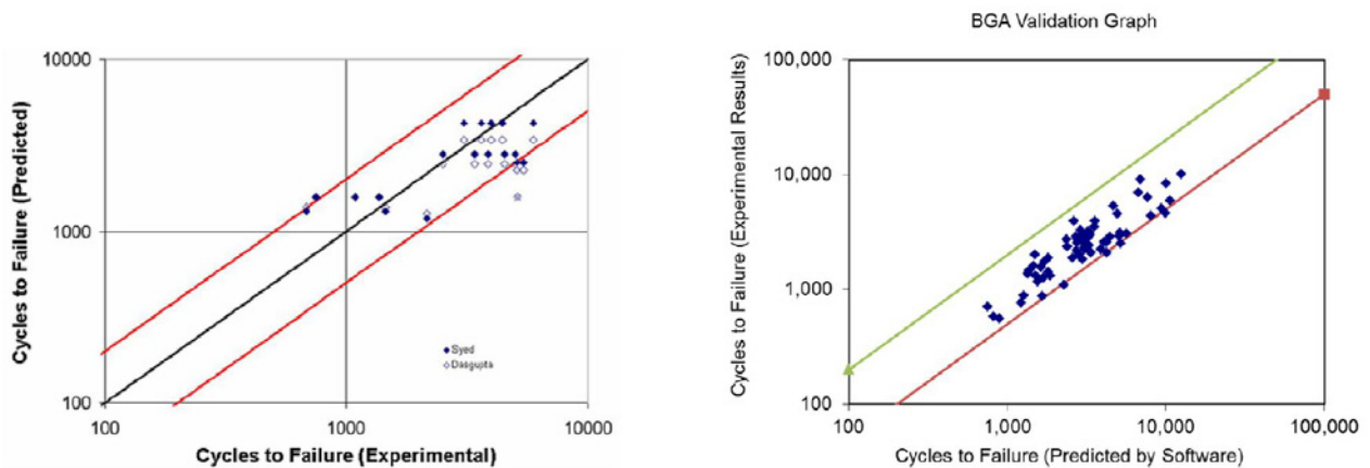
Figure 5. Validation graphs for chip components and ball grid array (BGA) packaging technology
