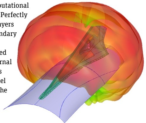
Ansys HFSS simulation results show radiation amplitude field generated by antenna designed within fuselage.
