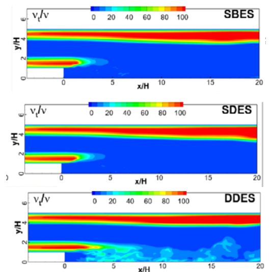
Figure 30. Contours of the eddy viscosity ratio for backstep.
