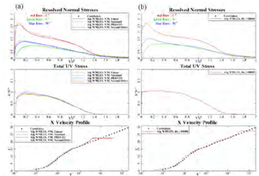
Figure 45. Profiles of resolved normal and shear Reynolds stresses and mean velocity in the flat plate boundary layer predicted by WMLES at two Reynolds numbers (a) Re_\theta=1000 with different numerical settings (b) Re_\theta=10000 with the second order pressure interpolation.
