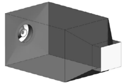
Figure 19. Computational domain for the ITS swirl burner.
