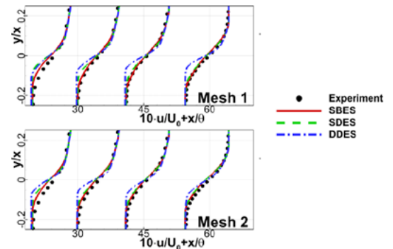
Figure 26. Profiles of the mean velocity profiles at different sections ( x/\theta_0 = 19.3, 29.6, 40.6, and 54.2 ) for mixing layer test case.
