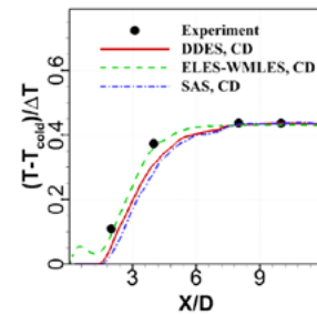
Figure 54. Comparison of the experimental and computational wall temperature distributions for T-Junction flow at the Front wall (90° - Figure 49) of the main pipe.
