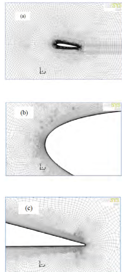
Figure 4. Details of the grid around a NACA 0012 airfoil (a) grid topology (b) Leading edge area (c) Trailing edge area.
