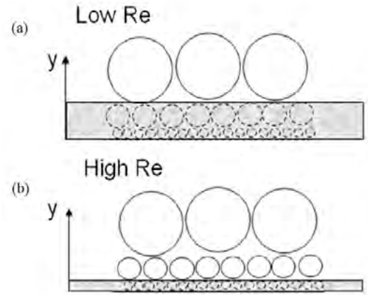
Figure 2: Sketch of turbulence structures for wall-bounded channel flow with viscous sublayer (a) Low Re number (b) High Re number (Gray area: viscous sublayer).
