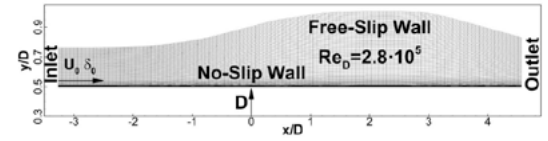
Figure 9. The domain and grid for the separated flow in CSO diffuser.
