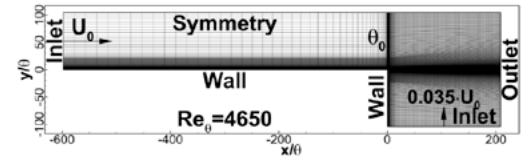
Figure 24. The domain and grid for the single stream mixing layer flow.
