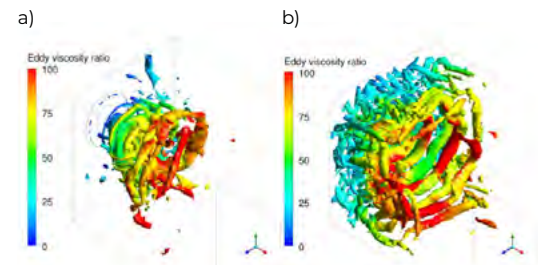
Figure 21. SAS solution for ITS combustion chamber, iso-surface Q=1/2(S^2-\Omega^2)=2 \times 10^7 \text{ s}^{-2} (a) non-reacting, (b) reacting flow.
