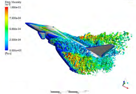
Figure 14. Turbulence structures for flow around a generic fighter aircraft (Q-criterion) as computed by SAS-SST model. Courtesy – EADS Germany GmbH – Military Air Systems DESIDER Project.
