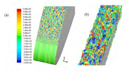
Figure 5. Turbulence structures of WALE LES computation around a NACA 0012 airfoil (a) Leading edge (b) Trailing edge (Q-criterion, color- spanwise velocity component).
