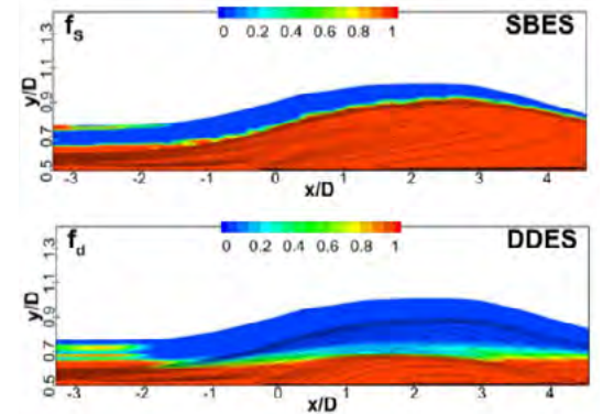
Figure 10. Contours of blending functions overset by vorticity iso-lines for CS=0 diffuser for SBES and DDES models.
