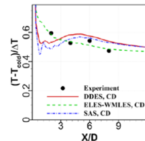
Figure 53. Comparison of the experimental and computational wall temperature distributions for T-Junction flow at the Top wall (0° - Figure 49) of the main pipe.
