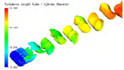
Figure 7. URANS computations of a flow past a circular cylinder (SST model).
