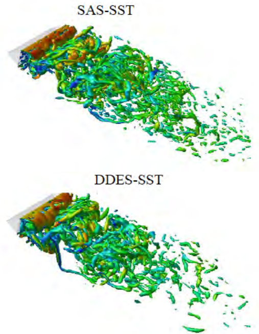
Figure 16. Turbulence structures for flow around a cylinder in crossflow.
