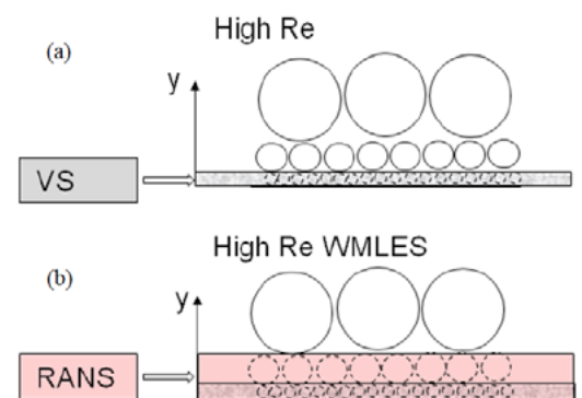
Figure 12. Concept of WMLES for high Re number flows (a) Wall-resolved LES. (b) WMLES.
