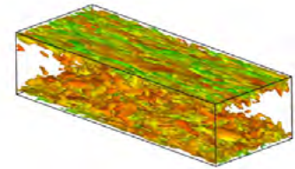
Figure 34. Turbulence structures for WMLES of channel flow at lowest Reynolds number ( Q=350 [s^{-2}] ).
