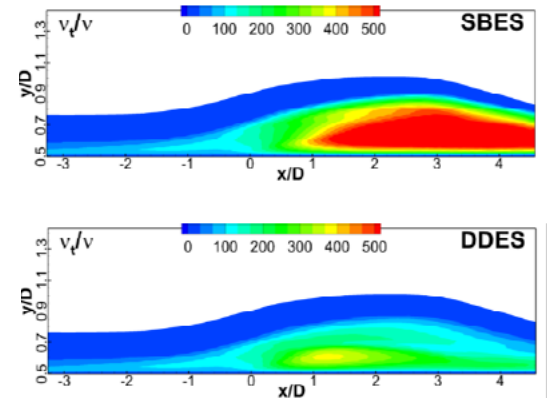
Figure 11. Contours of eddy viscosity ratio for CSO diffuser for SBES and DDES models.
