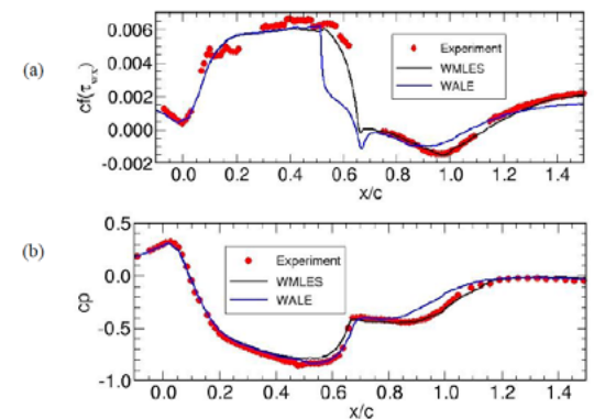
Figure 48. (a) Skin-friction, c_f , and (b) wall pressure coefficients, c_p , from NASA hump flow simulations. Comparison of WMLES and WALE LES methods in the LES domain.
