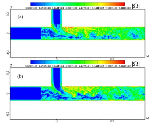
Figure 51. Vorticity contours for ELES/WMLES simulation (a) CD scheme (b) BCD scheme.
