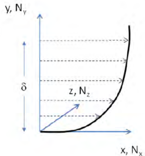
Figure 13. Sketch of boundary layer profile with thickness \delta . x -streamwise, y normal and z -spanwise.
