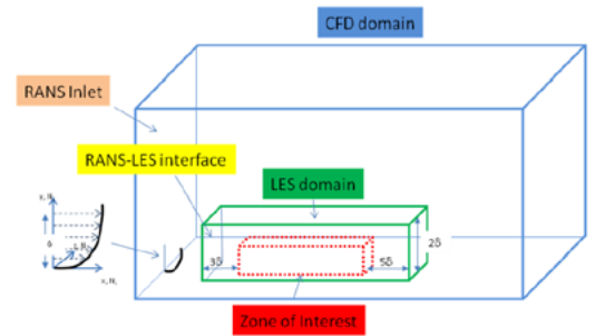
Figure 32. Sketch of embedded LES (ELES) domain.
