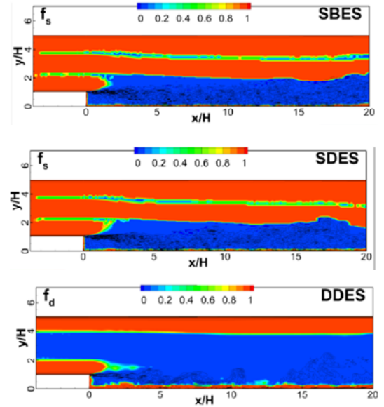
Figure 29. Contours of the blending function with the vorticity iso-lines for backstep.
