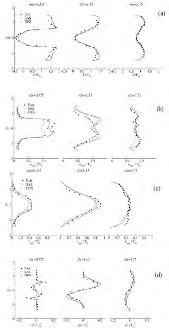
Figure 17. Velocity profiles and turbulence RMS profiles for three different stations downstream of the triangular cylinder ( x/a=0.375 , x/a=1.53 , x/a=3.75 ). Comparison of SAS-SST, DES-SST models, and experiment. (a) U-velocity, (b) u_{rms} , (c) v_{rms} , (d) u'v' .
