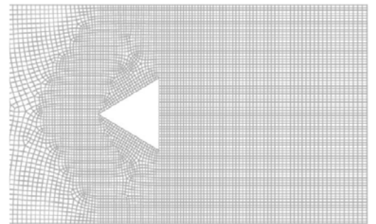
Figure 15. Grid around cylinder in crossflow.
