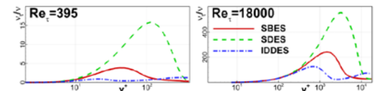
Figure 38. Profiles of the eddy viscosity ratio for different models.
